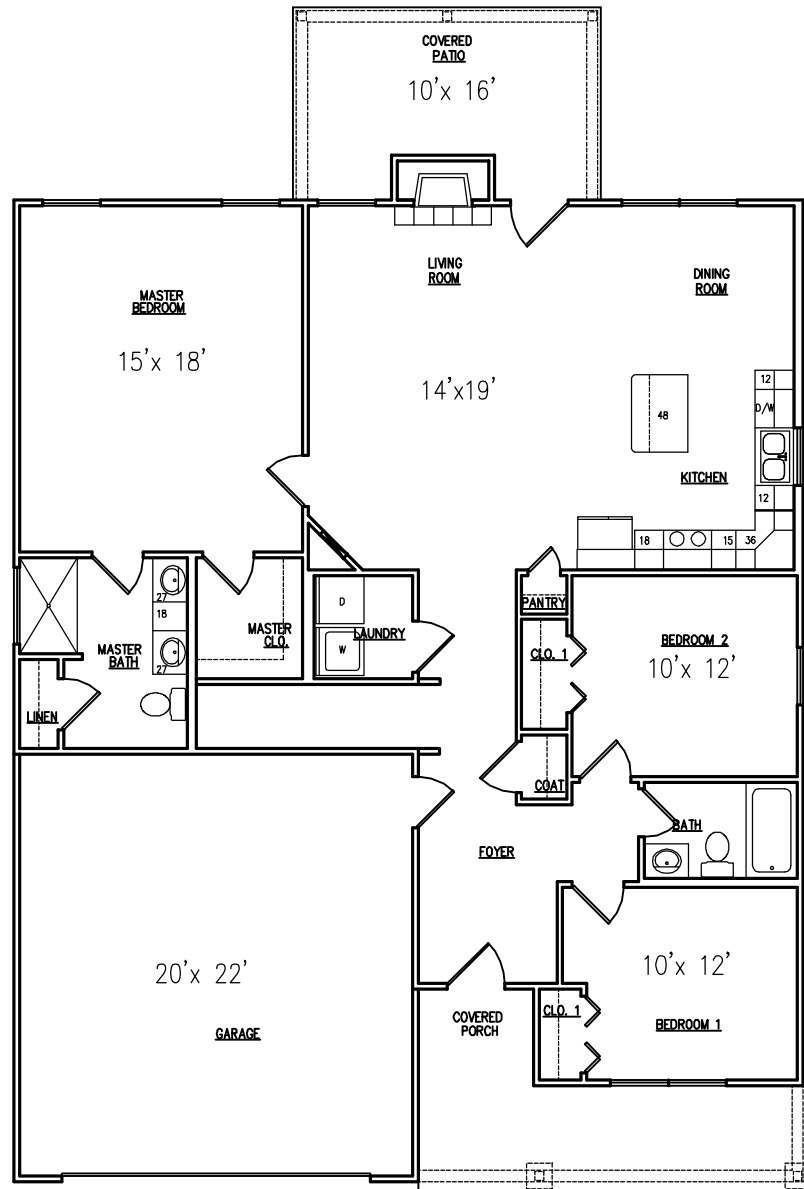
HUDSON FLOOR PLAN
